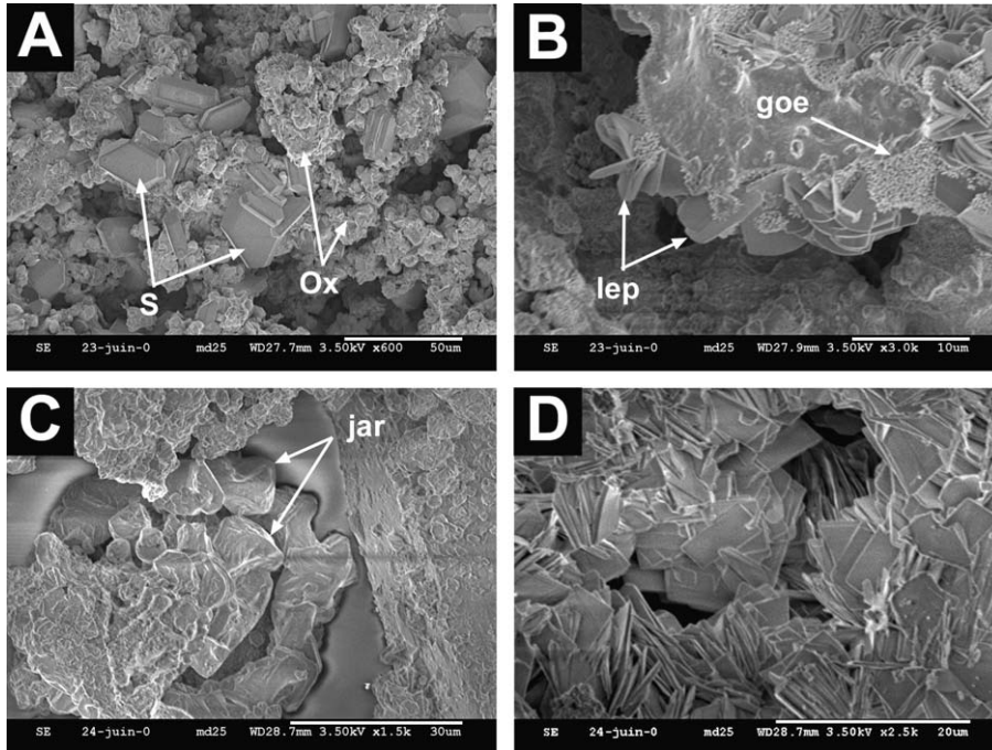
Fig. 15. SEM pictures of neoformed products on pyrrhotite control samples (w.a., water atmosphere; h.p.a., hydrogen peroxide atmosphere), (A) crystals of elemental sulfur (S) imbedded in iron (oxy)hydroxides (Ox); HPO in w.a. (B) Close view on iron (oxy)hydroxides showing relatively large platy crystals of lepidocrocite (lep) associated to nanocrystals of goethite (goe); MPO in w.a. (C) Crystalline aggregate of jarosite (jar); HPO in h.p.a. (D) Crystalline aggregate of copiapite tabular crystals; MPO in h.p.a.
