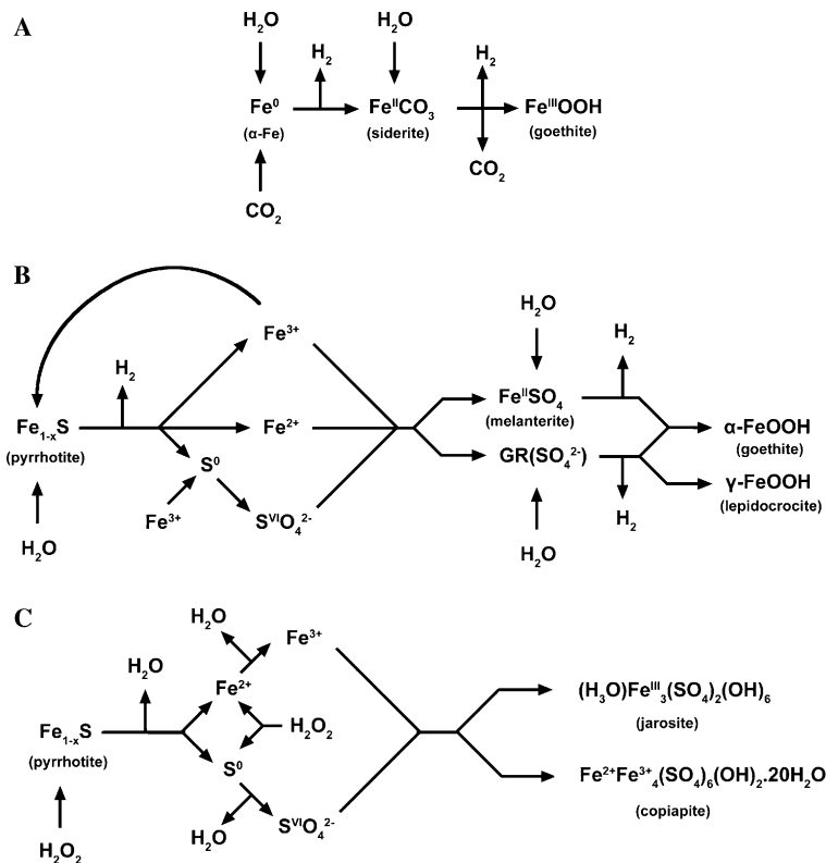
Fig. 16. Schematic summary of weathering reactions involved in our experiments. To improve clarity, only the main phases and chemical species have been represented. (A) Elemental iron \alpha\text{-Fe} in water atmosphere, (B) pyrrhotite in water atmosphere. GR designs green rust, (C) pyrrhotite in hydrogen peroxide atmosphere.
