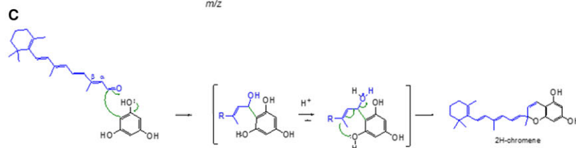
Fig. 7 Structural characterization of the chromene adduct. Representative ^1\text{H-NMR} (A) and MS spectra (B) of the 2H-chromene adduct are shown. ^1\text{H} NMR (500 MHz) and J -modulated ^{13}\text{C} NMR (125 MHz) spectra were obtained with \text{CDCl}_3 as solvent on a Bruker AVANCE II spectrometer. Chemical shifts are given in ppm with the solvent peaks for \text{CDCl}_3 at \delta_{\text{H}} 7.23, \delta_{\text{C}} 77 ppm, respectively. Coupling constants are reported in Hz. MS analysis was performed with LCQ Advantage mass spectrometer. ESI-MS was recorded on positive mode. (C) This 2H-chromene is the result of first, a 1, 2- C -addition of the free carbon atom of the resorcinol framework onto the carbonyl group of a RAL, followed by an intramolecular O -addition onto the \alpha - \beta double bond. (D) Retinal pigment epithelium (RPE) cells were incubated for 24 hrs with various concentrations of chromene. Cell viability was determined by MTT assay. The data are from a representative experiment repeated two times and presented as means \pm SD of sextuplicates.
