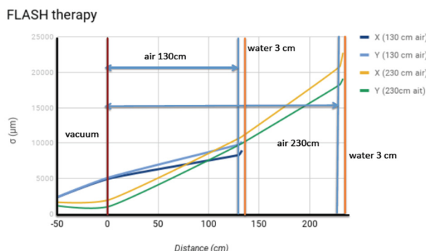
Figure 5: Beam widening for 70 MeV from end of vacuum window (0 in the horizontal scale), 130/230 cm air gap and 3 cm depth of water, calculated with BDSIM.
