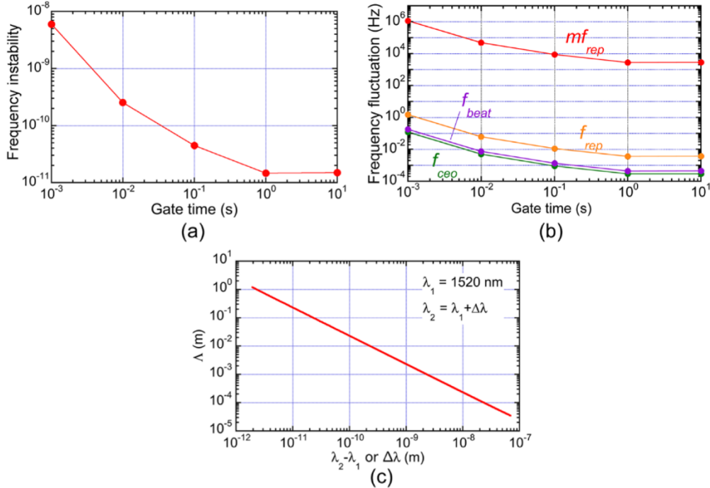
Fig. 4. Performance of the OFS. (a) Frequency instability of a rubidium frequency standard. (b) Frequency fluctuation of f_{ceo} , f_{rep} , f_{beat} , and mf_{rep} in the OFS. (c) Relation of the wavelength difference between two wavelength lights and the synthetic wavelength in the OFS.
