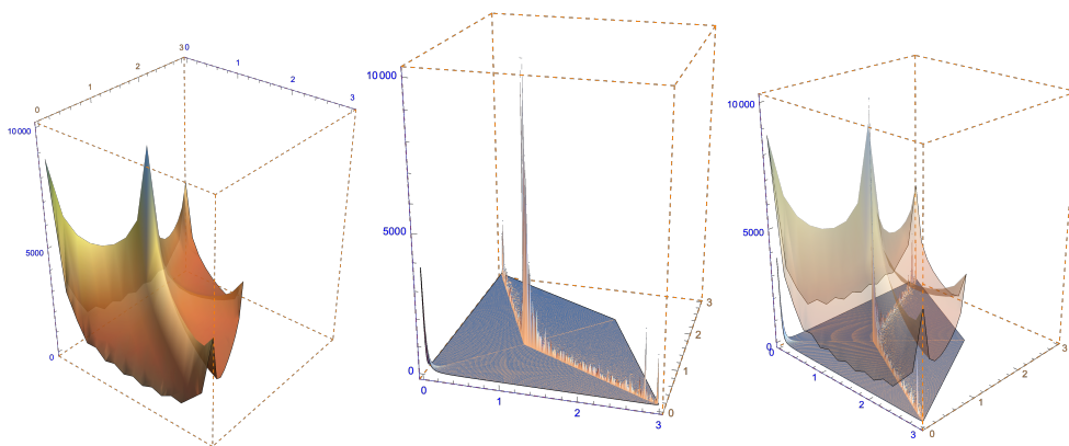
Figure 15: a) Semi-transparent surface approximating the vertically rescaled zonal structure constants of \chi_Z([8, 8])^2 . b) Point plot of the volume function J = \rho — because of the large vertical coordinate range, those parts of the surface lying far from the singularities look essentially flat and one only sees the singularities themselves (high values of J ). c) Superposition of a) and b). The horizontal coordinates (variables \nu = (\nu_1, \nu_2) running between 0 and 3) are the Dynkin coordinates corresponding to \alpha = \beta = \{1, 0, -1\} , obtained from the partition \{2, 1, 0\} after a global shift by -1 .
