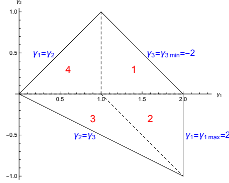
Figure 3: The four sectors in the Horn polygon of the quaternionic case for \alpha = \beta = \{1, 0, -1\} .
