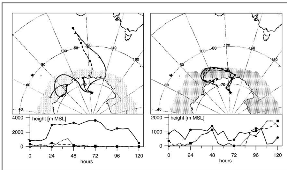
Figure 4. Example of 5 d backward trajectory in late July (left) and mid-September (right) when a moderate and strong sulfate depletion relative to sodium was observed on sea-salt aerosol at Concordia, respectively. Grey areas refer to the sea-ice cover. Dotted marks indicate the location every day. The plot are combined to corresponding monthly mean satellite derived sea ice map [Comiso, 1990, updated 2007] available on the Web at http://nsidc.org/ .
