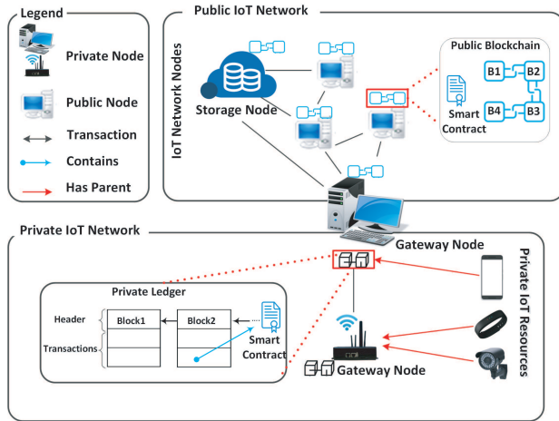
Fig. 1. PrivBlockchain Architecture
