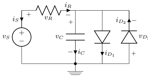
Figure 5: Diode Clipper circuit
