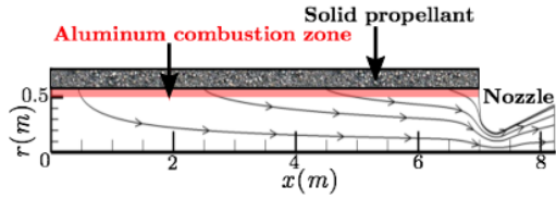
Fig. 1. Cylindrical solid rocket motor (SRM) geometry and computed gas streamlines in the numerical domain.
