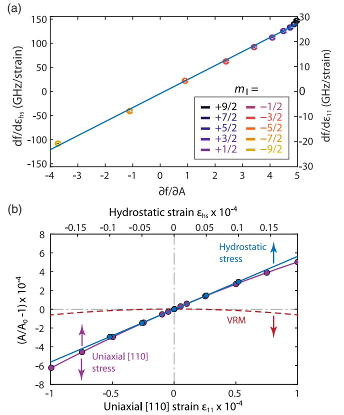
FIG. 3. (a) The gradient of the strain-induced frequency shifts ( df/d\epsilon ) for each of the ten Si:Bi ESR transitions is shown as a function of the first-order sensitivity of each transition to the hyperfine coupling ( \partial f/\partial A ). The linear relationship confirms the observed strain-induced shifts in Si:Bi result from tuning the hyperfine coupling, A , with a gradient \partial A/\partial \epsilon_{11} = 5.4 \pm 0.3 GHz or, equivalently, \partial A/\partial \epsilon_{\text{hs}} = 28.2 \pm 1.6 GHz. (b) Calculations showing the relative change in hyperfine coupling strength A/A_0 as a function of strain, comparing TB and valley repopulation models. To mimic the experiment, we show TB calculations of A/A_0 under uniaxial stress along [110] (purple curve and circles), which produces a hydrostatic component of strain ( \epsilon_{\text{hs}} , top axis) in addition to a uniaxial component along [110] ( \epsilon_{11} , bottom axis). This behavior can be understood by comparing with TB calculations for pure hydrostatic stress (blue curve and hexagons), plotted on the same axis of \epsilon_{\text{hs}} , as well as calculations from the VRM (red dotted curve), plotted on the same axis of \epsilon_{11} . The arrows indicate the relevant axes for each trace.
