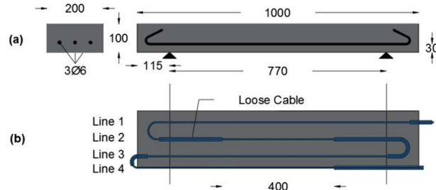
Figure 2 : (a) Shop drawing of tested beam and (b) instrumentation by optical cables.
