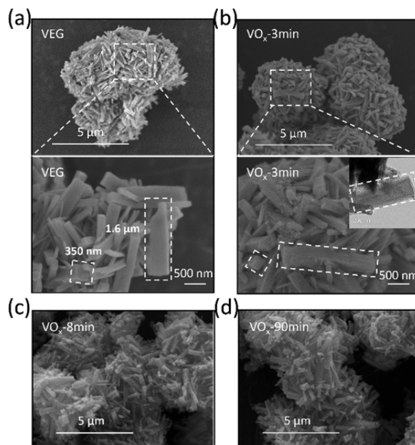
Figure 3. SEM images of (a) VEG, and its decomposed products at 300 °C for different times: (b) \text{VO}_x -3 min (inset shows the evident porosity from its corresponding TEM), (c) \text{VO}_x -8 min, and (d) \text{VO}_x -90 min.
