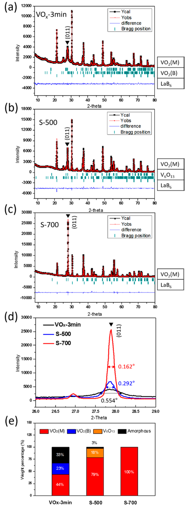
Figure 7. Typical Rietveld refinements of XRD data from (a) VO x -3 min; (b) S-500; (c) S-700; (d) comparison of XRD peak at 2\theta = 27.95^\circ preferred (011) orientation for VO 2 (M); (e) and the corresponding weight percentage of each component.
