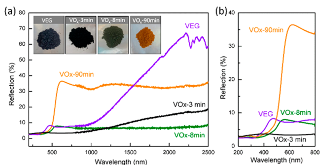
Figure 2. (a) The reflection spectra of the VEG, \text{VO}_x -3 min, \text{VO}_x -8 min, and \text{VO}_x -90 min samples in the wavelength region of 200–2500 nm; insets show photos of the VEG and \text{VO}_x samples; and (b) their reflection spectra in the visible region of 200–800 nm.
