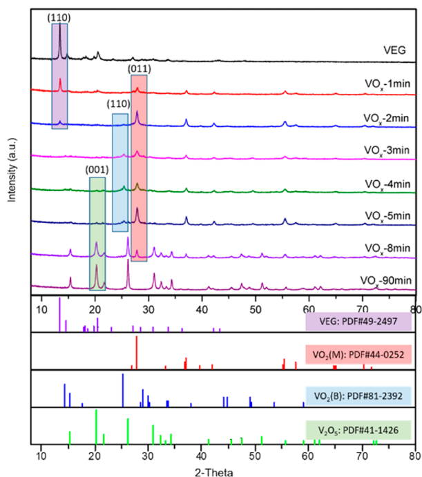
Figure 1. XRD patterns of samples synthesized by thermolysis of VEG precursor at 300 °C in air with different annealing times (1–5 min, 8 and 90 min). Corresponding PDF numbers provided at the bottom.
