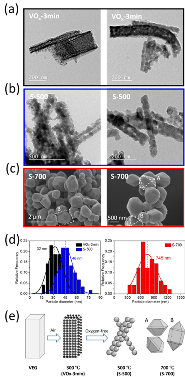
Figure 6. TEM and SEM images of the as-prepared \text{VO}_2 (M) particles synthesized with conditions (a) \text{VO}_x -3 min: 300^\circ\text{C} for 3 min in air through decomposition of VEG; (b) S-500: post annealing treatment of \text{VO}_x -3 min at 500^\circ\text{C} for 5 h in oxygen-free atmosphere; (c) S-700: post annealing of \text{VO}_x -3 min at 700^\circ\text{C} for 5 h in oxygen-free atmosphere. (d) Size distribution of the as-prepared \text{VO}_2 particles. (e) Schematic illustration of the morphological evolution for \text{VO}_2 particles. (A and B designate two kinds of deformed octahedra).
