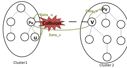
Fig. 2: Interfering nodes belonging to different clusters.
