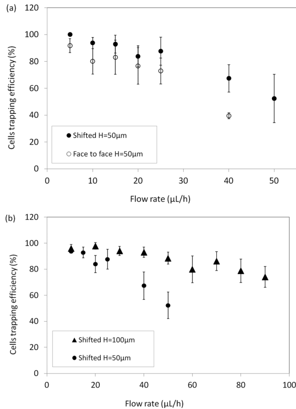
FIG. 7. Percentage of cells trapped on electrode as a function of flow rate (a) for the 2 designs and (b) for shifted electrodes with H = 50\ \mu\text{m} and 100\ \mu\text{m} (error bars represent mean deviation).
