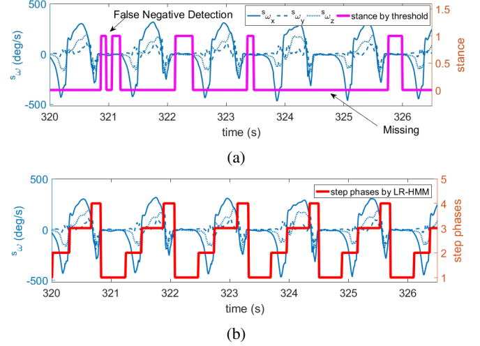
Figure 2: Step segmentation, jump 1 represents the stance phase. Stance detection by (a) a threshold method, where false negative detection and missing ones can be observed. (b) the proposed LR-HMM method.
