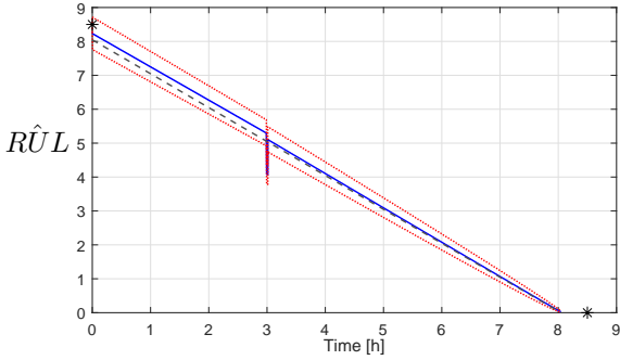
Fig. 6. Predicted RUL along the time: 1) by using the mean value of the estimated \alpha (solid line), 2) by using extreme values of the estimated \alpha (dotted line). Both compared with respect to the obtained RUL (dashed line). The symbol * represents the desired RUL.
