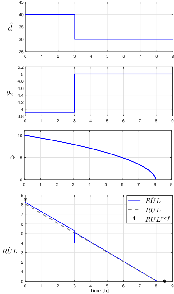
Fig. 7. System behavior under the effect of the RUL controller.
