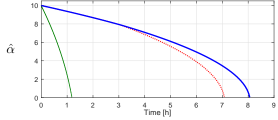
Fig. 9. Estimated contact quality coefficient \hat{\alpha} in presence of operation conditions changes and for three different cases: 1) without RUL control, 2) with a RUL control without updating the RUL prediction, and 3) with a RUL control which adapts the control actions according to the current RUL prediction.
