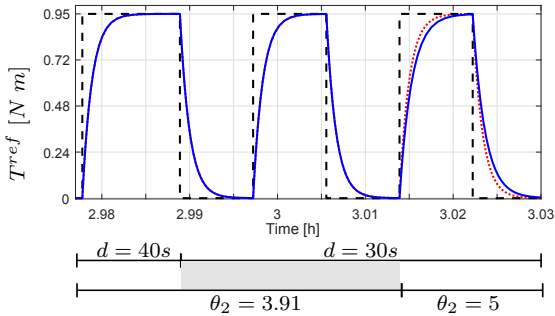
Fig. 8. The desired torque T^{ref} (dashed line) and the applied motor torque T_m (solid line). For comparison, the dotted line corresponds to the applied torque without updating the value of the parameter \theta_2 .
