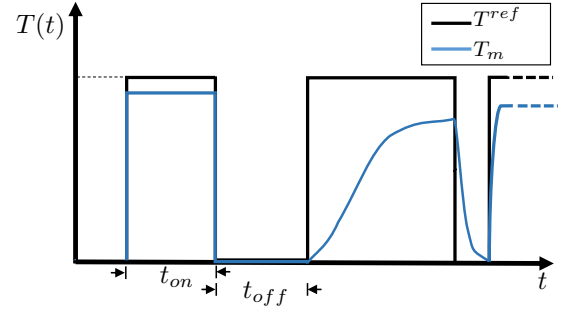
Fig. 3. Examples of applied motor torque T_m compared with respect to the desired one T^{ref} .
