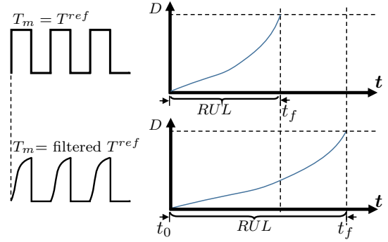
Fig. 1. Illustration of the obtained RUL for two different sequences of the motor torque. The obtained RUL increases in cases where the motor torque is a filtered (or smoothed) signal of T^{ref} .
