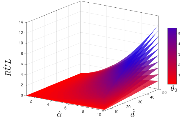
Fig. 5. Predicted RUL as function of the parameter \theta_2 , the estimated contact quality coefficient \hat{\alpha} and the operation conditions \hat{d} .
