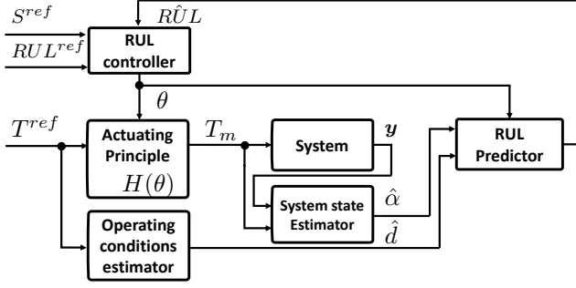
Fig. 2. Architecture for an optimal control of the RUL.
