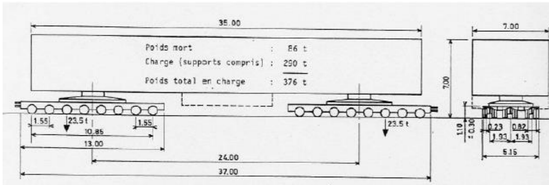
Figure 13: Convoy of type E.3 F.2
