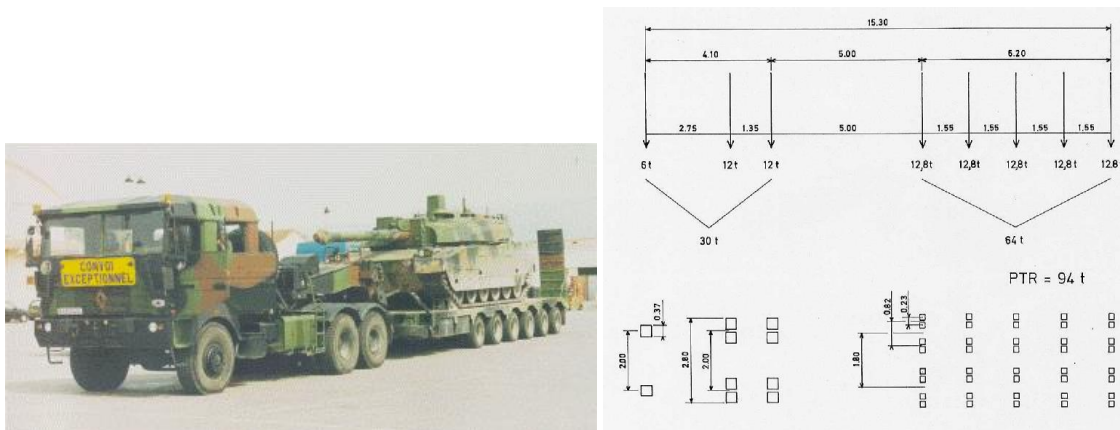
Figure 15: Military loads from a vehicle Leclerc.
