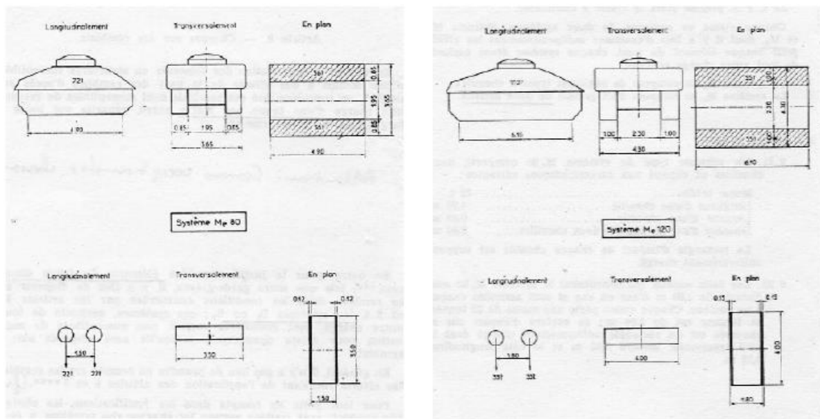
Figure 14: Military convoys MC80 (on the left) and MC120 (on the right).
