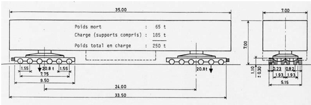
Figure 9: Convoy D.3 F.2
