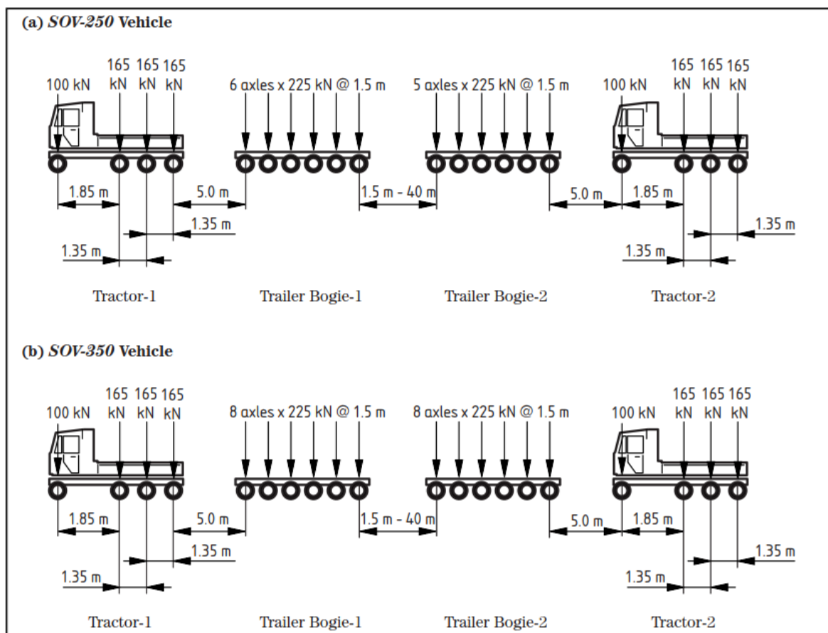
Figure NA.2 Basic longitudinal configuration of SOV model vehicles
