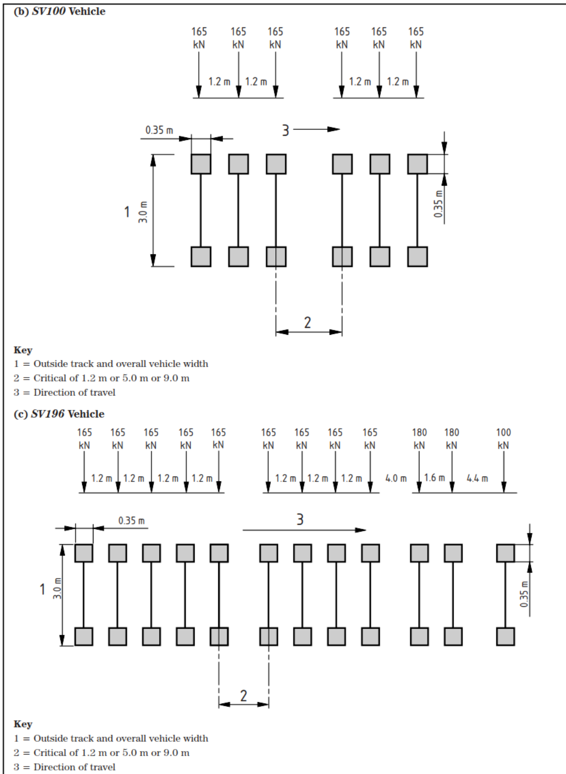
Figure NA.1 Basic longitudinal configuration of SV model vehicles (continued)
