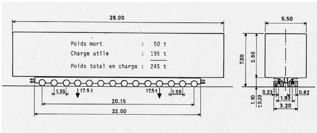
Figure 6: Convoy of type D.2 F.1
