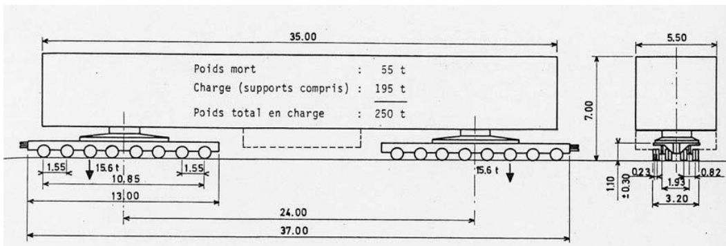
Figure 7: Convoy of type D.2 F.2
