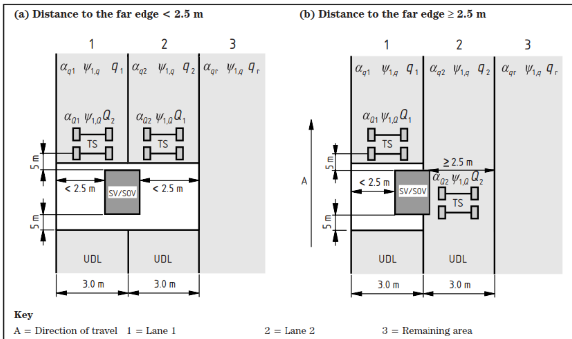
Figure NA.5 Typical application of SV or SOV and Load Model 1 loading when the SV or SOV vehicle straddles two adjacent lanes
