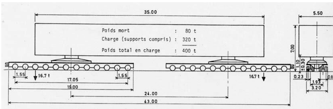
Figure 11: Convoy E.2 F.2
