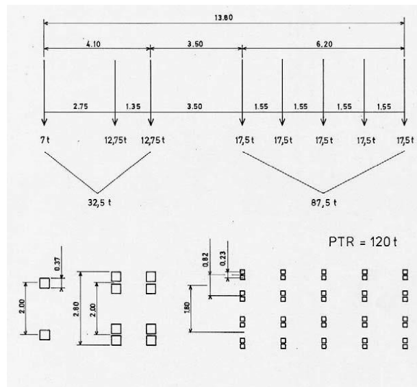
Figure 4: Convoy of type C1.
