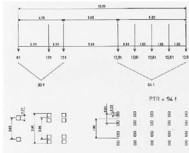
Figure 4: Convoy of type C1.
