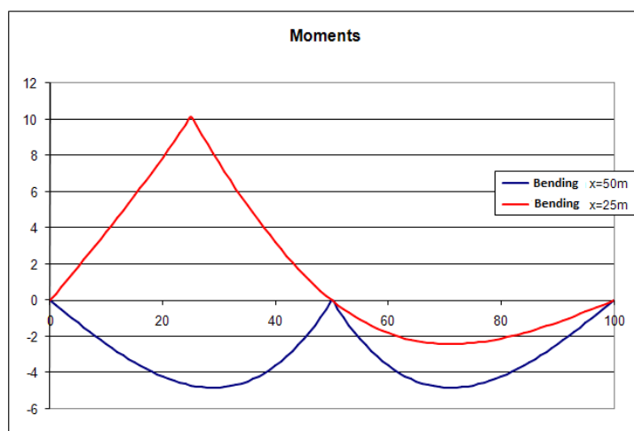
Figure 1: Example of influence line of bending moment at first mid-span ( x=25 metres) and on support ( x=50 metres), for a 2-span simply supported bridge, with both span length equal to 50 metres.
