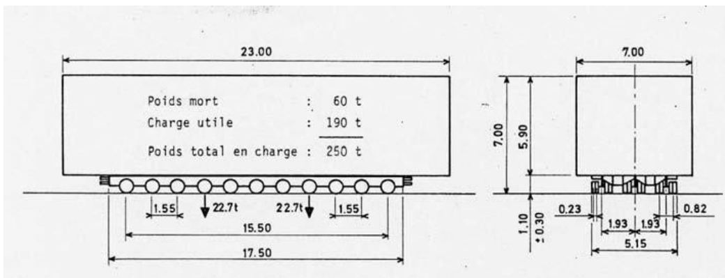
Figure 8: Convoy D.3 F.1
