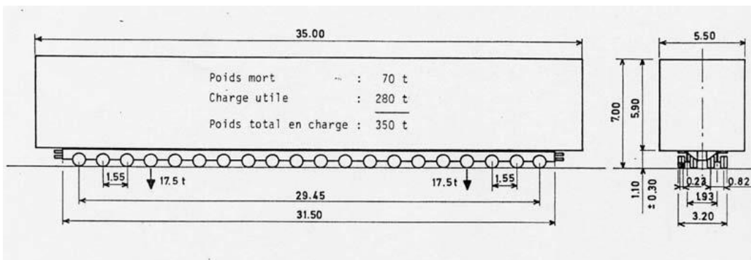
Figure 10: Convoy of type E.2 F.1
