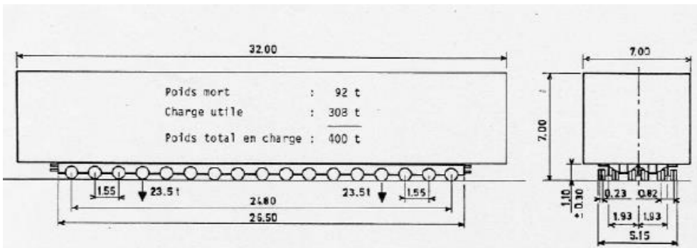
Figure 12: Convoy of type E.3 F.1
