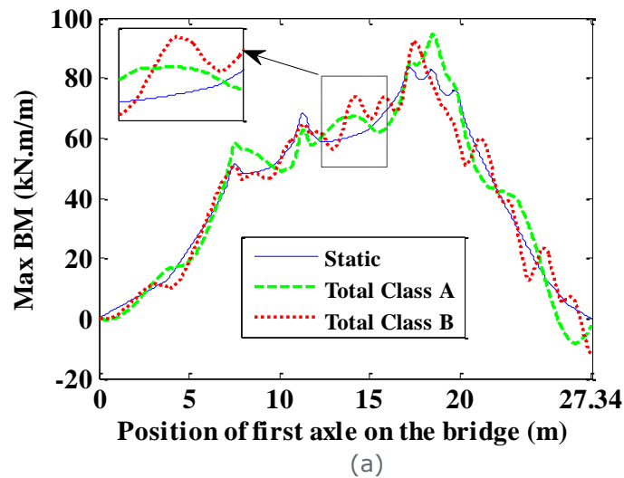
Figure 39. Static moment at section 'A-A' (kN.m/m) of Case_2 truck
