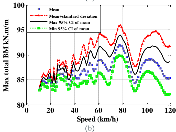
Figure 29. Total Bending Moment (BM) (kN.m/m) at the node holding maximum static value (i.e. node no. 18 in section 'A-A') versus speed of Case_0_b truck travelling over (a) class 'A' road profile (b) class 'B' road profile
