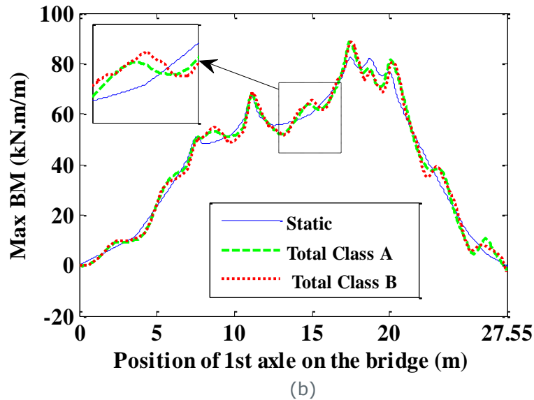
Figure 25. Static and total Bending Moments (BM) (kN.m/m) for class 'A' and class 'B' road profiles at the node holding maximum static value (i.e. node no. 18 in section 'A-A') versus position of first axle of Case_0_a truck travelling on the bridge at (a) critical speed, (b) 60 km/h
