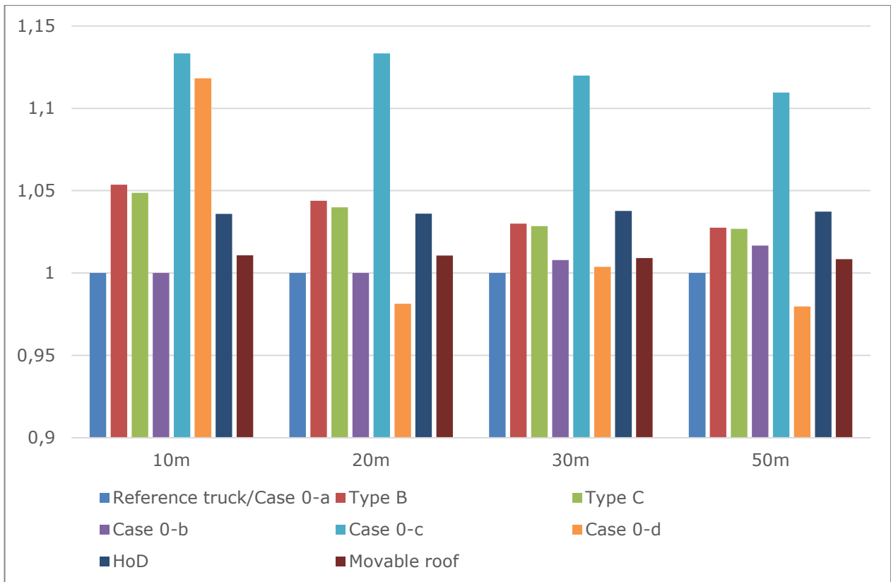
Figure 48: Ratio of extreme shear force at support 0 on the simply supported, two span bridge, for various length of span and the various vehicle configurations.
