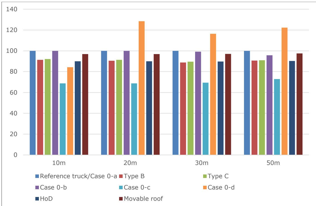
Figure 52: Fatigue life by considering the bending moment at mid-span 1 for the simply supported, two span bridge.
