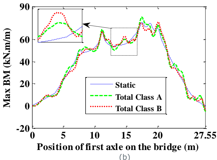
Figure 34. Static and total Bending Moments (BM) (kN.m/m) for class 'A' and class 'B' road profiles at the node holding maximum static value (i.e. node no. 17 in section 'A-A') versus position of first axle of Case_0_d truck travelling on the bridge at (a) critical speed, (b) 60 km/h
