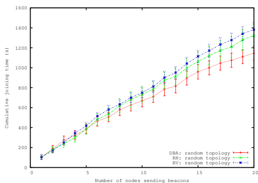
(b) Random topology.
