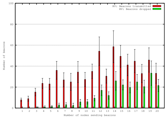
Figure 11: RV: Transmitted vs dropped beacons.
