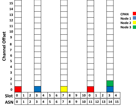
Figure 1: Transmission of beacons in DBA.
