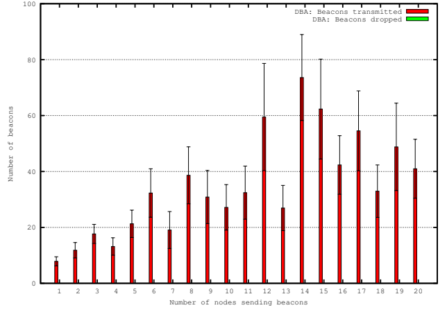
Figure 9: DBA: Transmitted vs dropped beacons.
