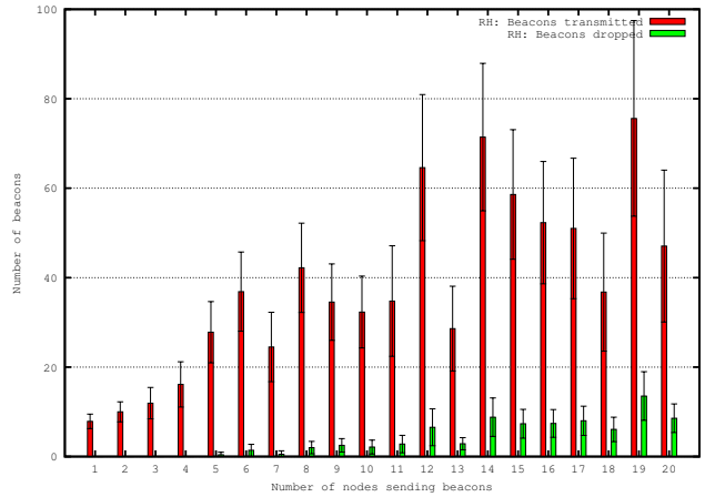
Figure 10: RH: Transmitted vs dropped beacons.
