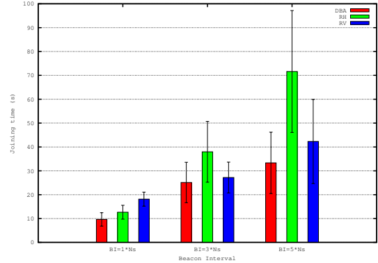
Figure 6: Joining time in a network of 20 nodes.
