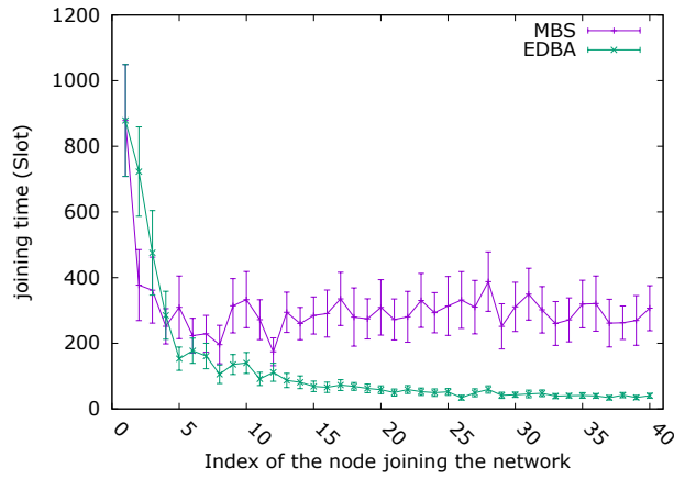
Fig. 7: The joining time obtained by MBS and EDBA for reliable links ( N_b=5 ).
