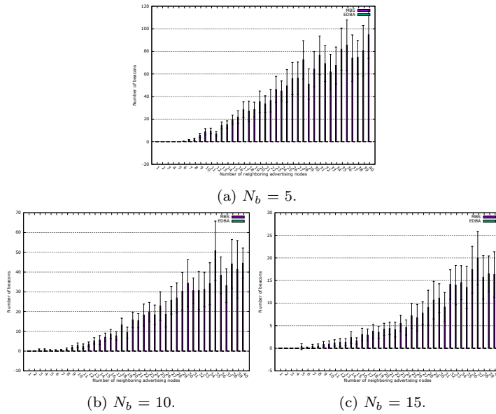
Fig. 11: Average number of beacons dropped
