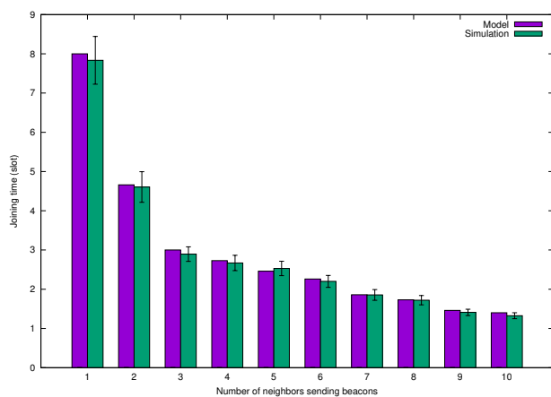
Fig. 5: Validation of the Markov model by NS3 simulations.
