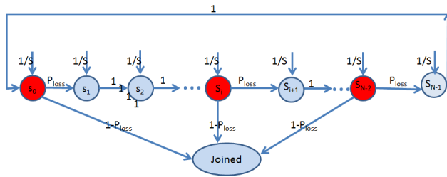
Fig. 4: The Markov model of a joining node with EDDBA.
