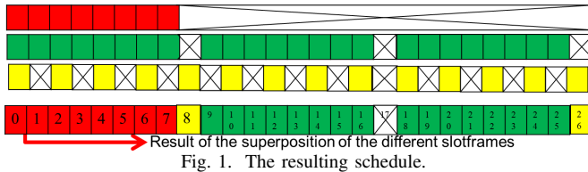
Fig. 1. The resulting schedule.
