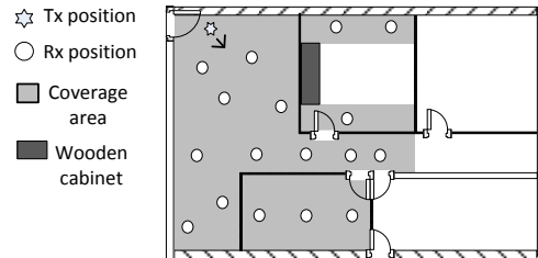
Fig. 8. Example of 802.11ad coverage area (no people).
