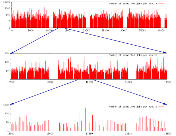
Fig. 6. Repetitive pattern in the job submission.
