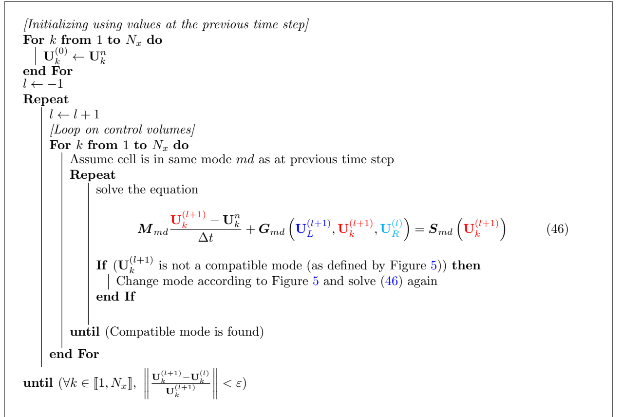
Algorithm 1: Fixed point for the implicitation of time integration
