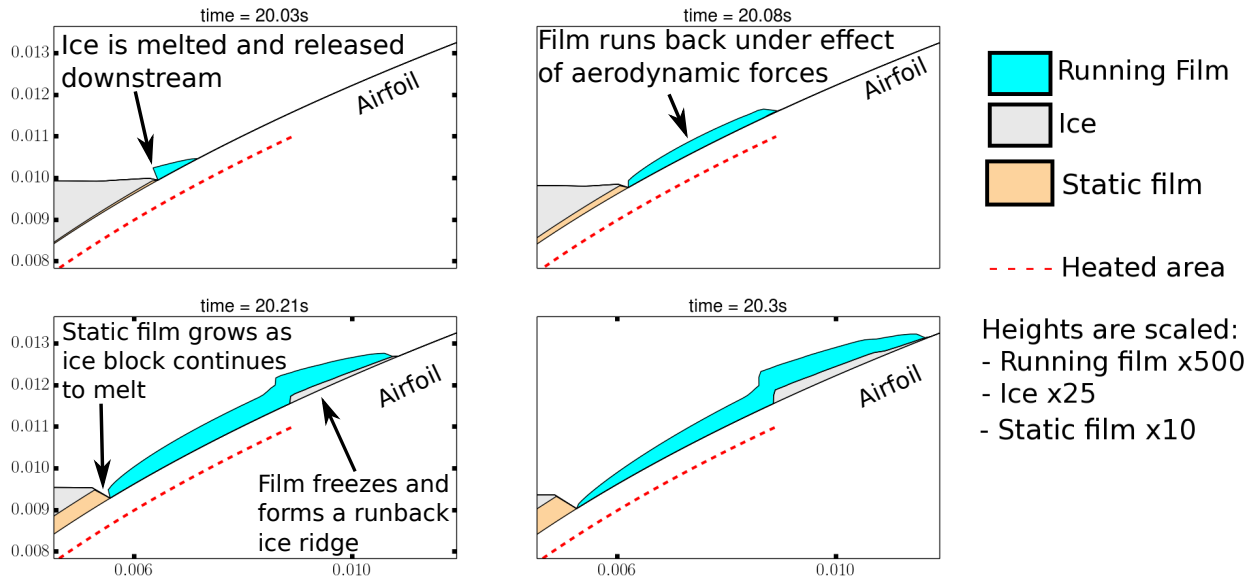
Figure 15: A small region of ice is melted. The resulting liquid water runs downstream.
