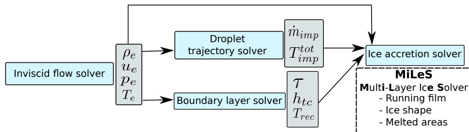
Figure 1: State of the art icing code architecture. The work presented in this paper focuses on the ice accretion solver.
