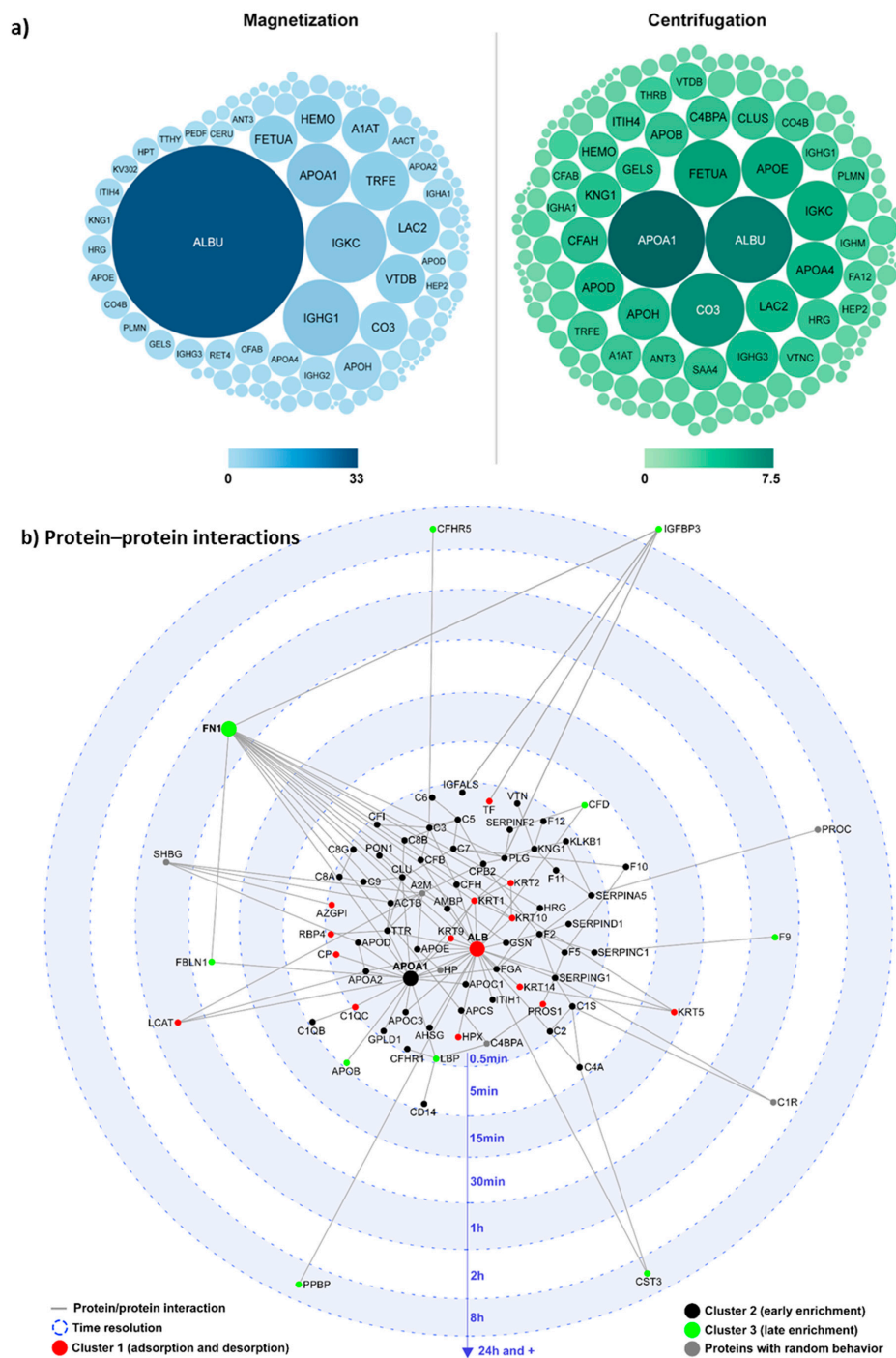
Figure 2. (a) Different proteomic profiles of the protein corona after Fe_3O_4@MSN separation by magnetization (blue) or centrifugation (green). Sizes and colors of human protein clues are proportional to their relative percentage within the corona. The 35 highest abundant proteins are labelled. The color scale unit is Normalized Spectral Abundance Factor (%). Reproduced from Pisani et al. 2017 [17] with permission from the Royal Society of Chemistry. (b) Protein–protein interactions are represented in a network developed using the NetworkAnalyst software [18,19], based on InnateDB [20]. The target represents the time scale (0.5 min to 7 days). Each protein (represented by its gene symbol) is placed according to its time of appearance within the corona. The colors indicate the cluster membership. The grey lines represent the protein–protein interactions. Proteins that have a lot of interactions with other proteins are represented by a larger visual cue. Reproduced from Pisani et al. 2017 [5] with permission from the Royal Society of Chemistry.
