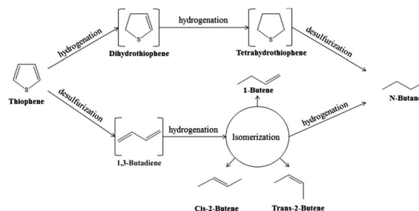
Scheme 1 Main reaction pathway for thiophene hydrodesulfurization.
