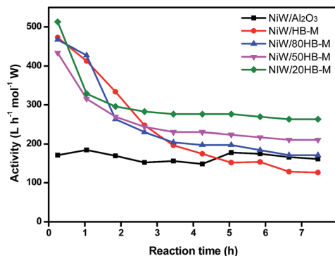
Fig. 10 Catalytic activity of mixed catalysts with time-on-stream in HDS of thiophene.
