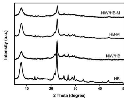
Fig. 1 X-ray diffraction patterns of various samples.
