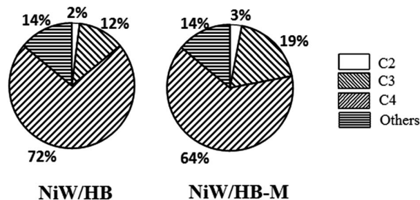
Fig. 9 Product selectivity of NiW/HB and NiW/HB-M at steady-state in HDS of thiophene.
