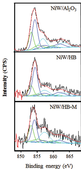
Fig. 5 Emission region of Ni2p XPS spectra of various catalysts sulfided at 673 K with their fit decomposition curves: experimental (black), simulation (red), Ni x S y (green), NiWS (blue), Ni 2+ (cyan).
