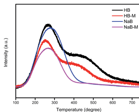
Fig. 11 NH 3 -TPD profiles for various samples.
