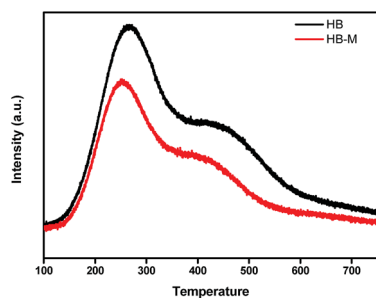
Fig. 3 NH 3 -TPD profiles for HB and HB-M.
