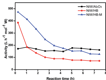
Fig. 8 Catalytic activity of various catalysts with time-on-stream in HDS of thiophene.
