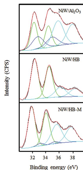
Fig. 4 Emission region of W4f XPS spectra of various catalysts sulfided at 673 K with their fit decomposition curves: experimental (black), simulation (red), WS 2 (green), WO x S y (blue), W 6+ (cyan).
