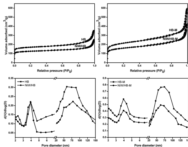
Fig. 2 N 2 sorption isotherms and pore distribution of various samples.
