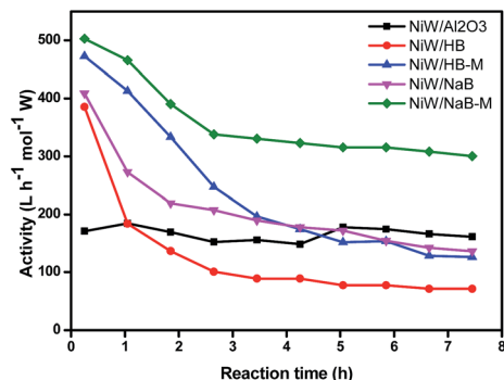
Fig. 12 Catalytic activity of various catalysts with time-on-stream in HDS of thiophene.
