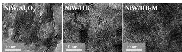
Fig. 6 HRTEM images of sulfided NiW/Al 2 O 3 , NiW/HB and NiW/HB-M.
