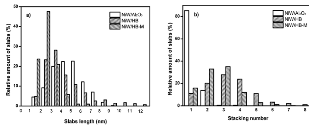
Fig. 7 Distribution of the length (a) and stacking number (b) of the WS 2 slabs over various supports.
