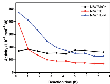
Fig. 8 Catalytic activity of various catalysts with time-on-stream in HDS of thiophene.
