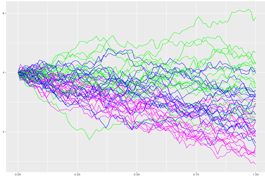
FIGURE 1. Illustration of the classification problem with 3 classes (blue, green and magenta) for the three different values of \theta^* for model Additive with n = 100 , N = 100 .
