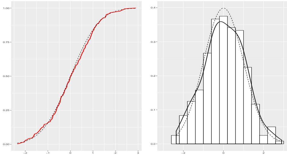
FIGURE 3. Illustration of the asymptotic normality of \hat{\theta} . Left: estimated cumulative distribution function of Z := \sqrt{N}(\hat{\theta} - \theta^*) (solid curve) and the theoretical one (dotted curve). Right: histogram of Z_i 's with the estimated density (solid curve) and the theoretical one (dotted curve), with N = 1000 , n = 1000 .
