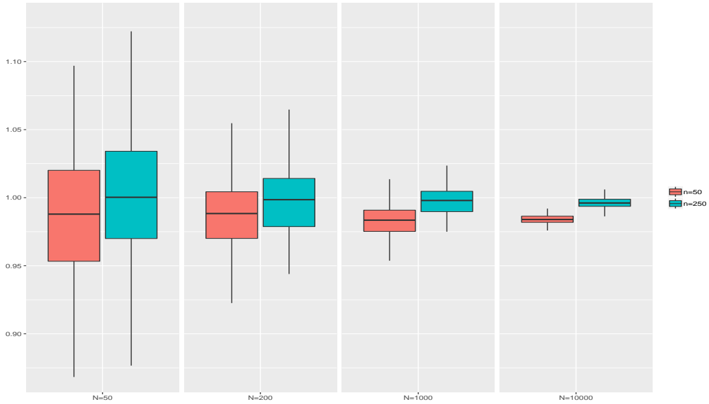
FIGURE 2. Boxplots for the MLE estimators of \theta^* = 1 in the additive OU model 1 as a function of parameters n and N .
