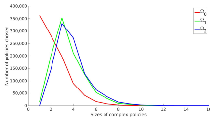
Fig. 4: Number of policies selected per policy size for three increasingly more complex outcome spaces by the IM-PB learner
