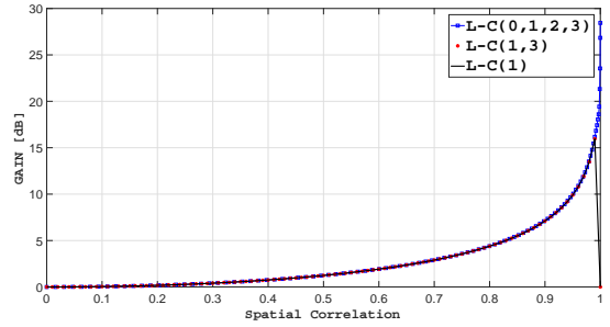
Fig.4 G_B as a function of \alpha , circular Bernoulli impulsive interference.
