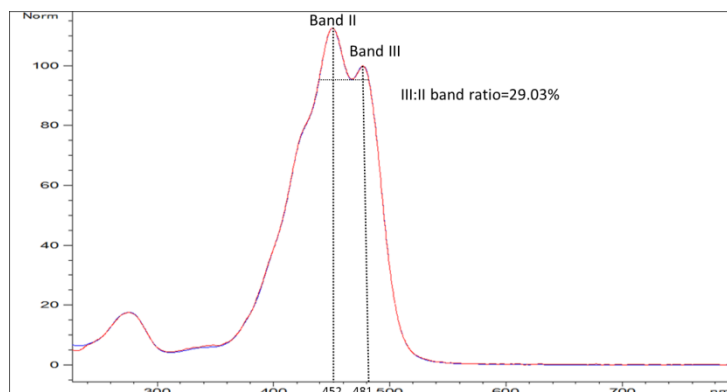
Fig.2. Identification of the pigment eluting at 24.582 min as zeaxanthin (1) based on absorption spectrum, maximal absorbance wavelengths and III:II band ratio.
