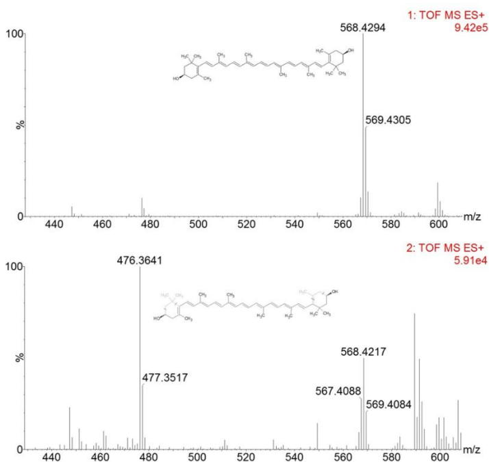
Fig.3. MS E fragmentation pattern of zeaxanthin ( 1 ) isolated from Porphyridium purpureum .
