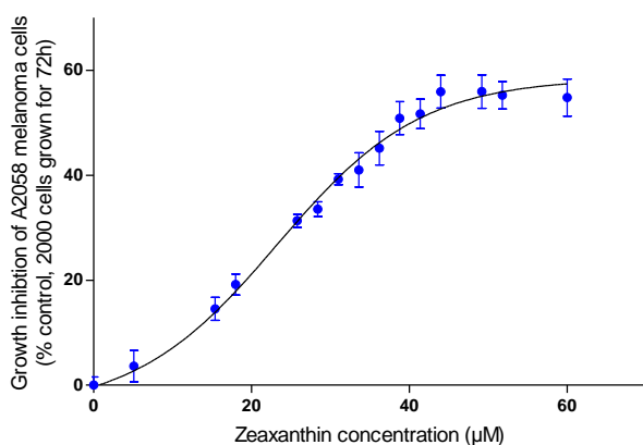
Fig. 4. Growth inhibition of A2058 cell in the presence of zeaxanthin ( 1 ). A2058 cells were grown for 72 h in a cell culture medium containing increasing concentrations of zeaxanthin. The antiproliferative activity of zeaxanthin was observed for concentrations superior to 5 \mu M and IC 50 was determined as 40 \mu M.
