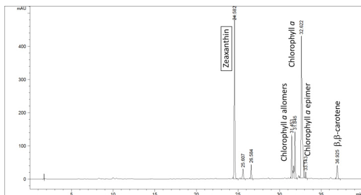
Fig.1. RP-HPLC Chromatogram of Porphyridium purpureum ethanol extract at 436 nm obtained using the Van Heukelem and Thomas analysis (van Heukelem et al., 2001). The pigment profile was identical to that previously reported in Serive et al. (2017).
