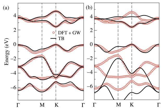
FIG. 4. DFT+ GW and TB calculations for electronic energy dispersion in \text{MoS}_2 . (a) The fit of TB model of Ref. [24], (b) the fit of TB model of Ref. [26]. The zero energy was aligned to the top of the valence band v .
