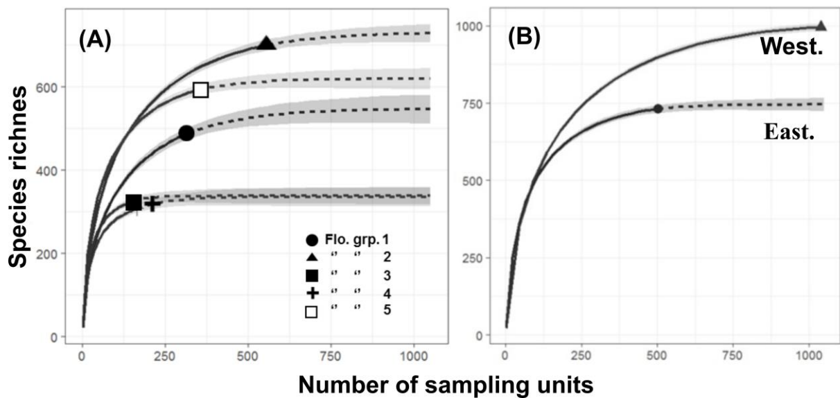
Figure 2 -- Comparison of plant species richness associated to carob trees according to (A) the five floristic groups of table 1, (B) Western and Eastern Mediterranean. Sampling-unit-based rarefaction (solid lines) and extrapolation (dashed lines) curves are shown with 95% confidence intervals (grey-shaded regions).
