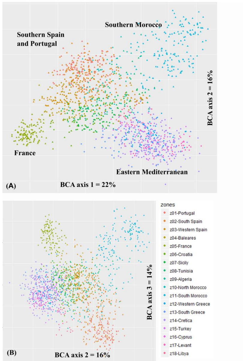
Figure 1 -- Ordination of the 1542 relevés describing plant assemblages associated with the carob tree based on the Bray-Curtis dissimilarity index and a between-class analysis (BCA) with the geographical areas as the class factor. The relevés are coloured according to their geographical area. The BCA was performed on the 100 first components of a principal coordinate analysis (PCoA). BCA is accounting for 19% of the total inertia coming from the PCoA and the three first BCA axes are accounting for 52 % of BCA inertia. A permutation test confirmed the significance of the structure bore by BCA ( p = 0.001 , 999 permutations).
