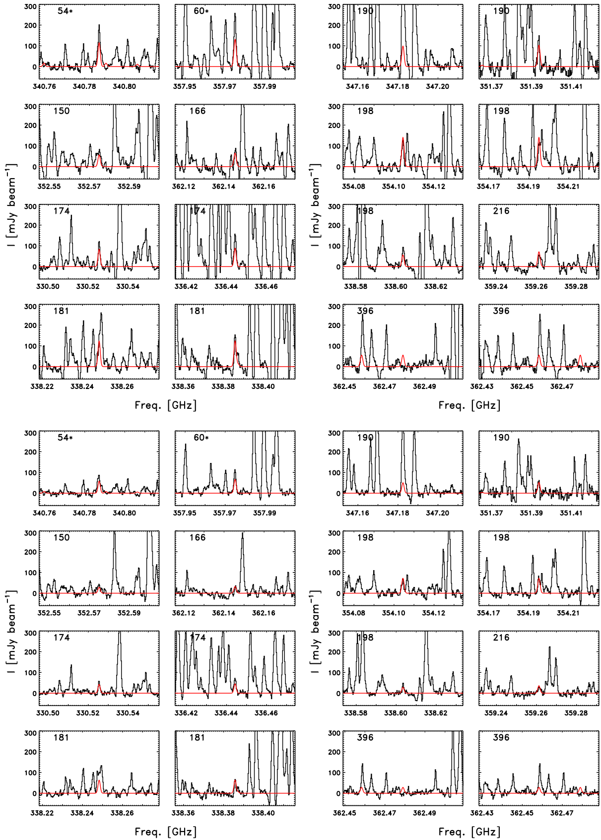
Fig. B.8. As in Fig. B.1, 16 brightest lines of \alpha -CH 3 CHDOH toward the half-beam ( upper panel ) and full-beam ( lower panel ) offset positions. The asterisks next to the upper energy level in some panels indicate features for which the multiple transitions (from the same species) overlap.
