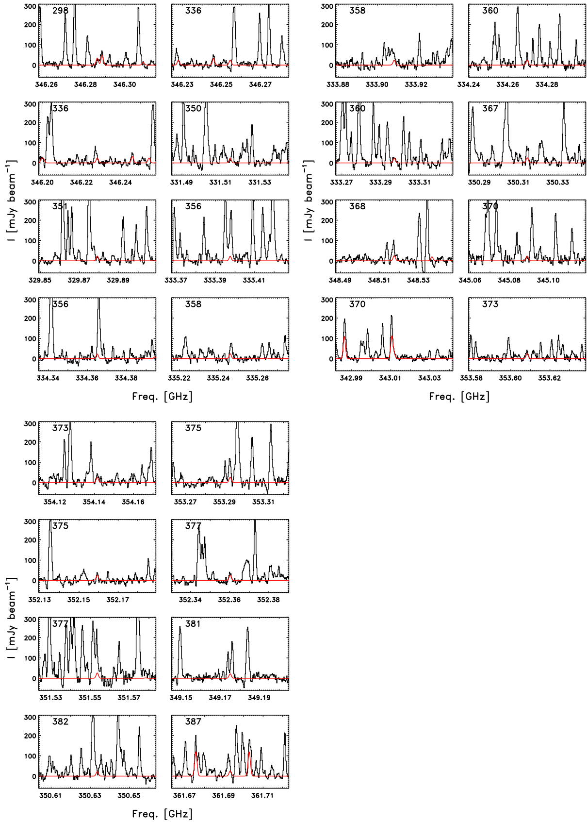
Fig. B.21. As in Fig. B.1, 24 brightest lines of the second ^{13}\text{C} isotopologue of acetaldehyde, \text{CH}_3^{13}\text{CHO} , as expected from the synthetic spectrum.
