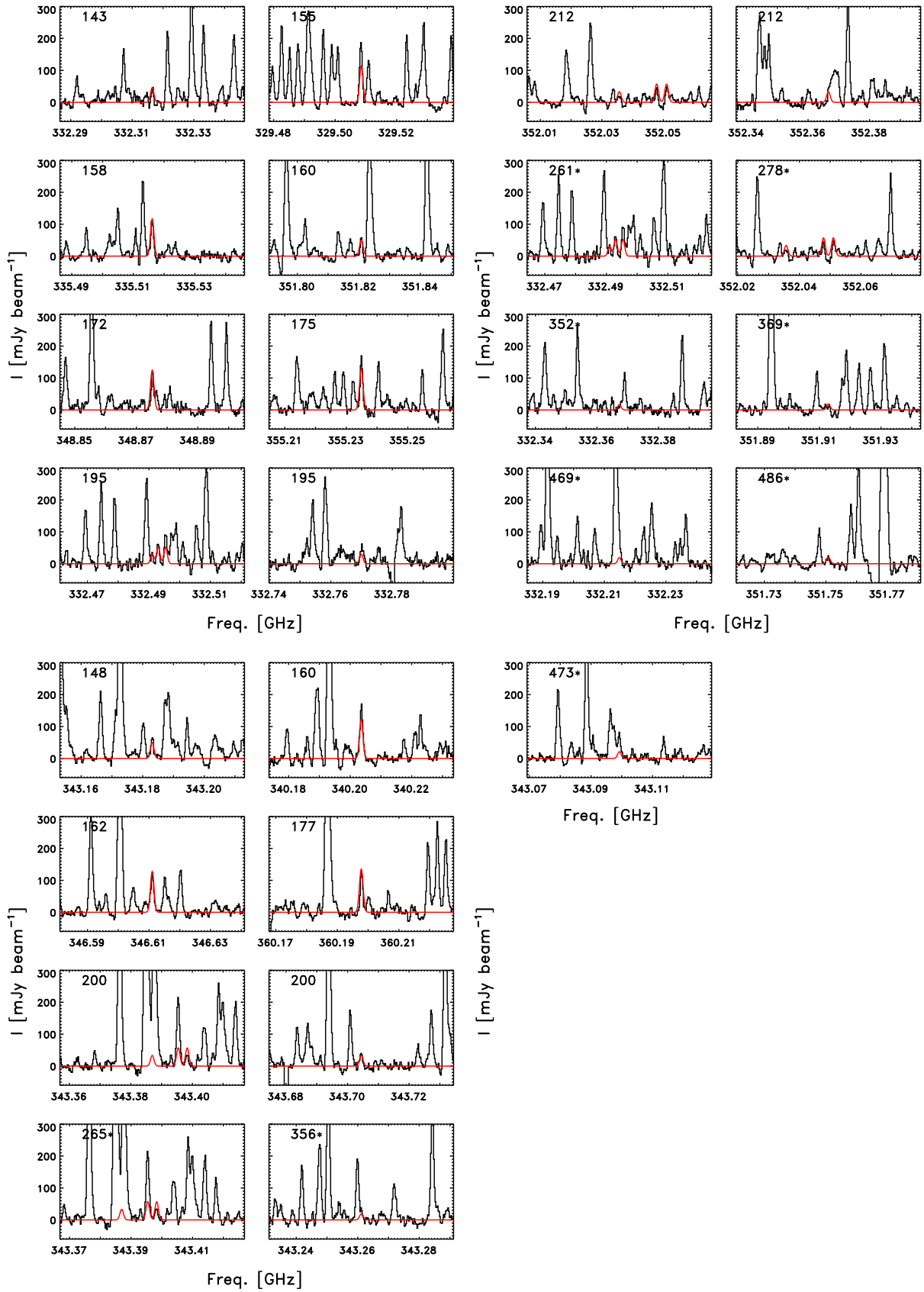
Fig. B.15. As in Fig. B.1, the brightest lines of the ^{13}\text{C} -isotopologues of ketene with ^{13}\text{CH}_2\text{CO} shown in the upper panels and \text{CH}_2^{13}\text{CO} in the lower panels .
