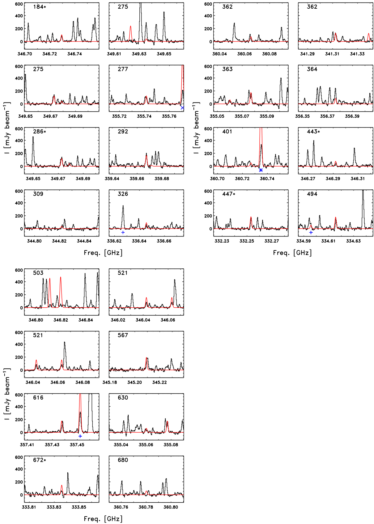
Fig. B.4. The 24 brightest optically thin lines of CH 2 DOH as expected from the synthetic spectrum toward the full-beam offset position. In the cases, where other lines fall in the band that are strongly optically thick at 50 or 300 K, they have been marked with a plus-sign or cross, respectively. The discrepancies for the lines at 349.62 and 346.82 GHz likely reflect issues with the catalogue entries for these high excitation transitions.
