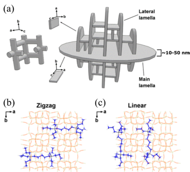
Figure 2. (a) Schematic illustration of the MFI framework and a hierarchically intergrown zeolite. (b) Optimized structures of the Pr 6 -diquat-C 5 /silicalite-1 complexes when the spacer of the molecules is located in the zigzag and linear pores, respectively. The axes indicate the crystallographic axis of the MFI framework.
