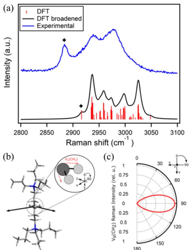
Figure 3. (a) Spontaneous Raman spectrum of Pr 6 -diquat-C 5 in a MFI zeolite and theoretical spectra (discrete and broadened using Lorentzians with a fwhm of 5 cm -1 ) of the free molecule having an optimized geometry simulated by DFT calculations. (b) Illustration of the CH 2 stretching vibrational mode of the theoretical spectrum. The arrows drawn on the molecule and the schematic representation of the CH 2 group indicate the atomic motions associated with the vibrational mode. (c) Normalized polarization dependence of the vibrational mode depicted in panel b, with angles relative to the axis formed by the spacer (indicated by the y axis).
