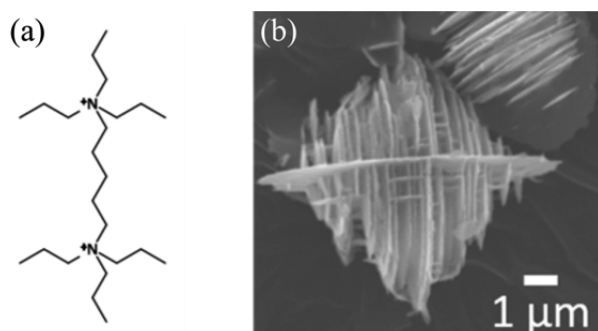
Figure 1. (a) Chemical structure of Pr 6 -diquat-C 5 . (b) SEM image of a typical hierarchically intergrown silicalite-1 crystal obtained using Pr 6 -diquat-C 5 as a templating agent.
