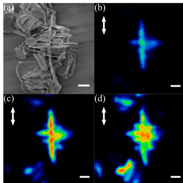
Figure 4. (a) SEM image of hierarchical silicalite-1 crystals (scale bar = 1 μm). (b–d) SRS images at 2884 cm -1 of the OSDA molecules inside the micropores of the crystal, at 1, 3, and 5 μm from the top of the crystal (scale bar = 1 μm). The excitation lasers have a linear polarization parallel to the main lamella (indicated by the arrow).
