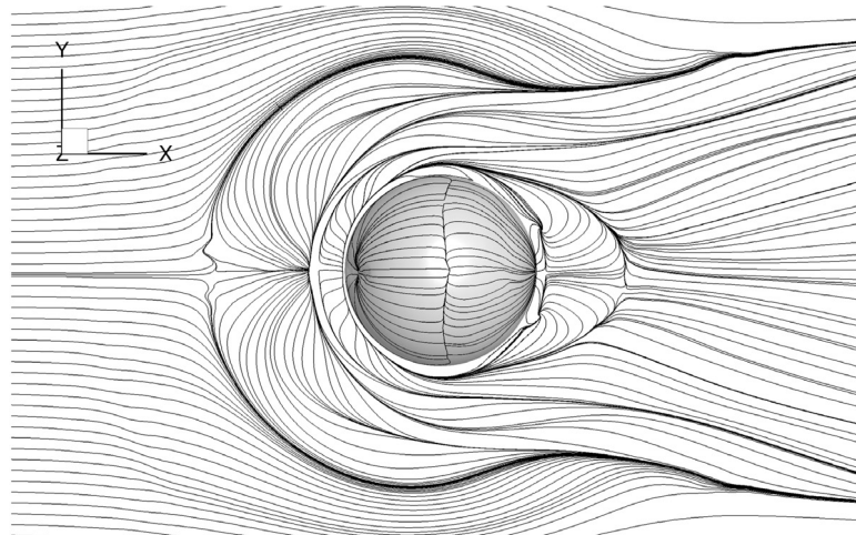
(c) Re = 100,000 .
