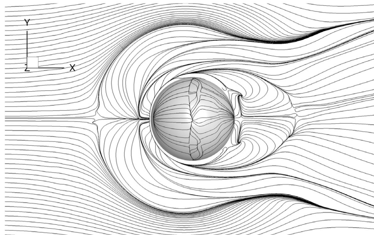
(a) Re = 50,000 .
