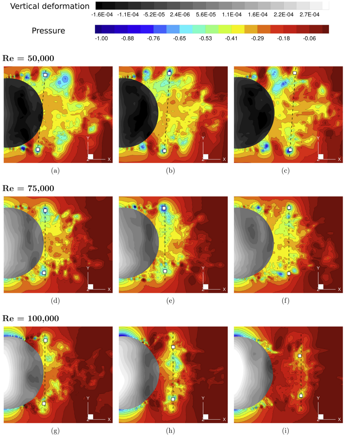
Fig. 17. Visualization of the instantaneous vertical deformations normalized by U_\infty^2/(2g) and of the vortical structures (fluid pressure coefficient c_p = (p - p_\infty)/(\rho_{\text{air}} U_\infty^2/2) near the bottom wall) at the back of the flexible hemisphere in case of the symmetric shedding type for three instants in time; symmetric arc-type vortices are highlighted by square symbols.
