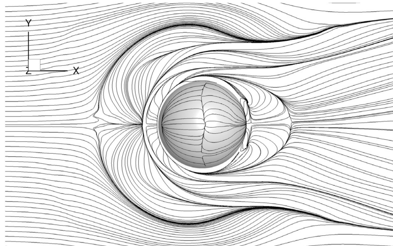
(b) Re = 75,000 .
