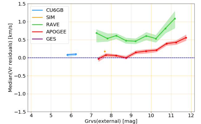
Fig. 11. Top panel: median radial velocity residuals as a function of the external G_{\text{RVS}}^{\text{ext}} magnitude. Middle panel: median radial velocity residuals as a function of the internal G_{\text{RVS}}^{\text{int}} magnitude. Bottom panel: median radial velocity residuals as a function of the external G_{\text{RVS}}^{\text{ext}} magnitude for a subset of giant stars. The lower and upper 1\sigma uncertainties on the measures of the medians are represented as shaded areas.
