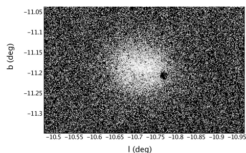
Fig. 4. Only a few regions are under-scanned due to the lack of on-board resources, such as here, on the edge of NGC 6541.
