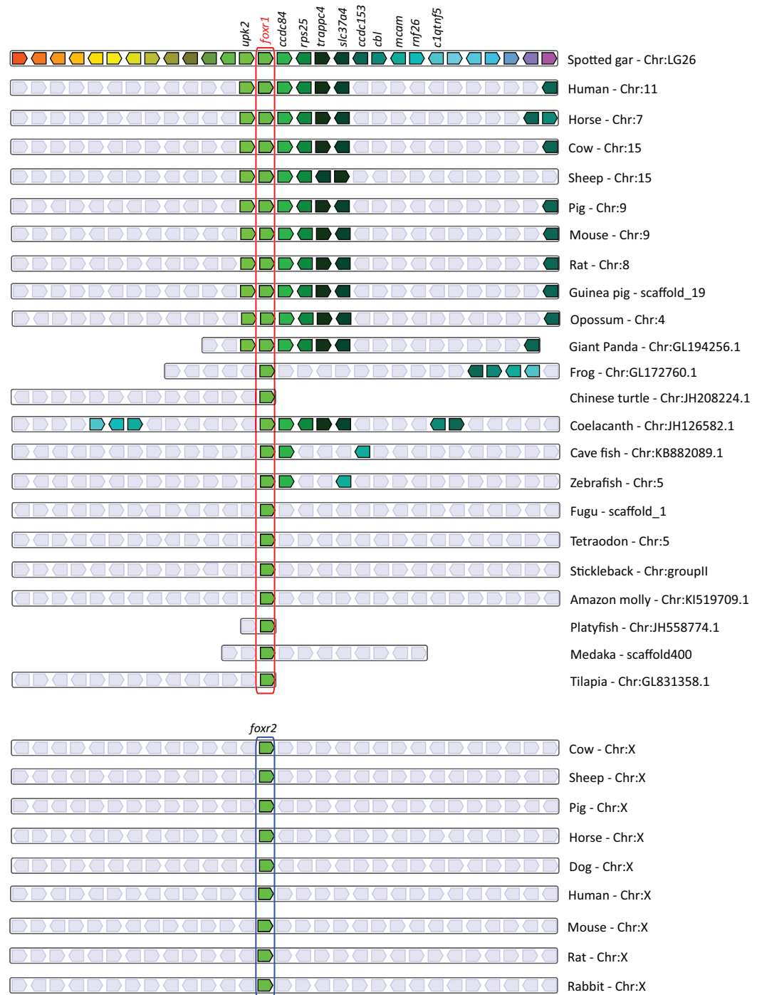
Figure 2 Conserved genomic synteny of foxr1 genes. Genomic synteny maps comparing the orthologs of foxr1 , foxr2 , and their neighboring genes, which were named after their human orthologs according to the Human Genome Naming Consortium (HGNC). Orthologs of each gene are shown in the same color, and the chromosomal location is shown next to the species name. foxr1 orthologs are boxed in red while foxr2 orthologs are boxed in blue. Light gray boxes denote the lack of synteny of the corresponding genes in the indicated species as compared to gar.
