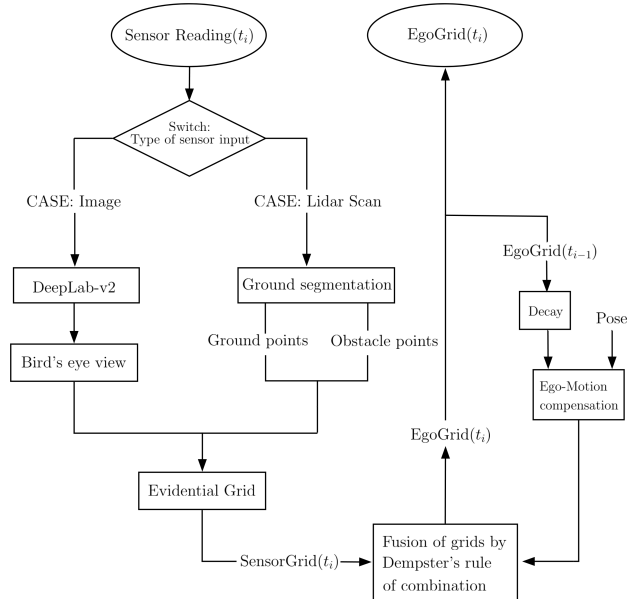
Fig. 1: Asynchronous fusion based algorithm. Images and LIDAR scans are individually processed once acquired. An evidential grid is then built from the sensor input, and fused with the current global grid, or EgoGrid, based on the current vehicle pose. Thus, no LIDAR/camera synchronization is needed.
