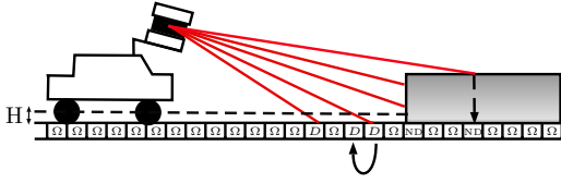
Fig. 2: Evidential mapping from a LIDAR scan. The state having the largest mass is reported for each cell. The curved arrow indicates the occurrence of backward propagation.
