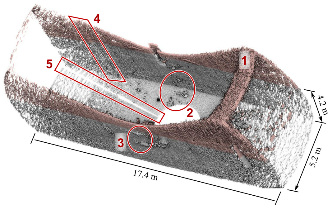
Figure 8. Rendering of a raw sonar output (from a single scanning position on the lock chamber floor). 1: artifacts due to surface reflections (coloured in salmon). 2: acoustic anomalies in the water column. 3: acoustic phenomena due to signal backscattering. 4: acquisition anomaly probably due to a temporary blocking of the horizontal rotation system. 5: lack of measurement.
