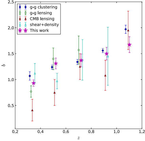
Figure 10. Bias obtained from second-order CiC, including systematic uncertainties from Section 6, compared with the two-point correlation study (Croce et al. 2016), the CMB–galaxy cross-correlation study (Giannantonio et al. 2016), galaxy–galaxy lensing (Prat et al. 2018), and the shear + density analysis (Chang et al. 2016). The points for the same z have been separated in the horizontal axis for visualization purposes.
