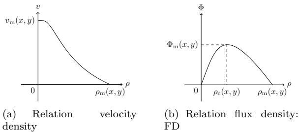
Figure 3: Speed and flow vs. density.
