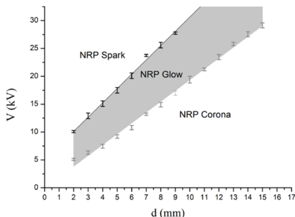
Fig. 1. Domain of existence of the NRP glow regime for a given set of parameters ( v = 3.4 m/s, f = 10 kHz).
