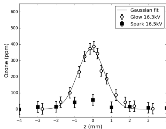
Fig. 3. Radial distribution of ozone density in the post-discharge (17 mm downstream of the electrodes) in the NRP glow (16 kV) and spark (16.5 kV) regimes. Spatial resolution: 300 \mu m.
