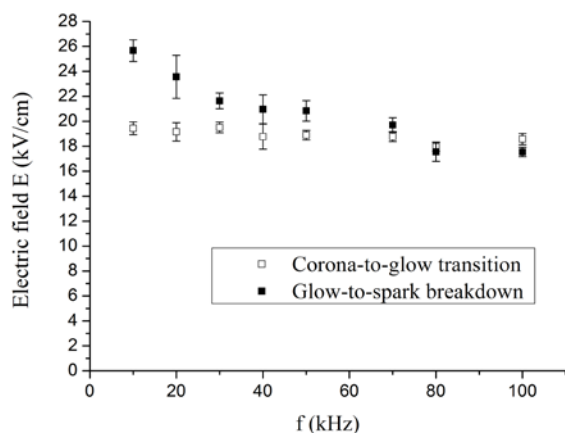
Fig. 2. Transition electric fields (Corona-to-glow and Glow-to-spark) as a function of repetition frequency. Air velocity is kept constant at 3.4 m/s.
