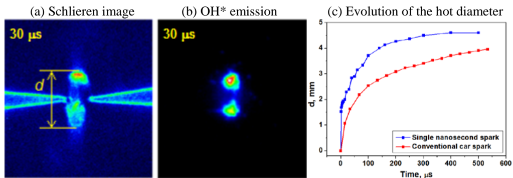
Figure 3. Comparison of a) Schlieren image and b) distribution of spontaneous \text{OH}^* emission (308 nm) at 30 \mu\text{s} after a single nanosecond spark in air at P=1 atm, with a 10 ns pulse of amplitude U=36 kV, \epsilon=6 mJ; c) Evolution of the hot core diameter d ; Nanosecond spark (blue curve): U=36 kV, 10 ns pulse, deposited energy: \epsilon=6 mJ. Conventional automotive spark (red curve): \epsilon=55 mJ. Distance between pins: 1 mm.
