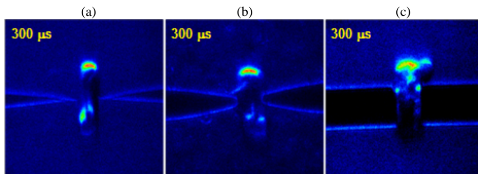
Figure 4. Schlieren images obtained for a single nanosecond spark in air at P=1 atm, U=36 kV for different electrode systems: a) conic stainless steel pin with 30- \mu\text{m} radius of curvature tips; b) paraboloid tungsten pins with tapered 150- \mu\text{m} tip radius; c) cylindrical tungsten electrodes of diameter 2 mm. The distance between the electrodes is 1 mm. The horizontal knife edge cuts 90 % of light.
