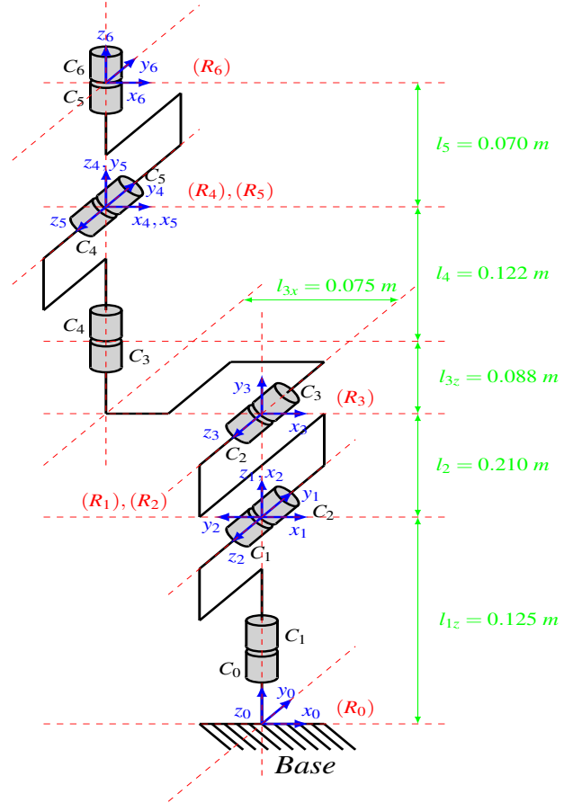
Figure 2: Robot frames for MDH convention.
