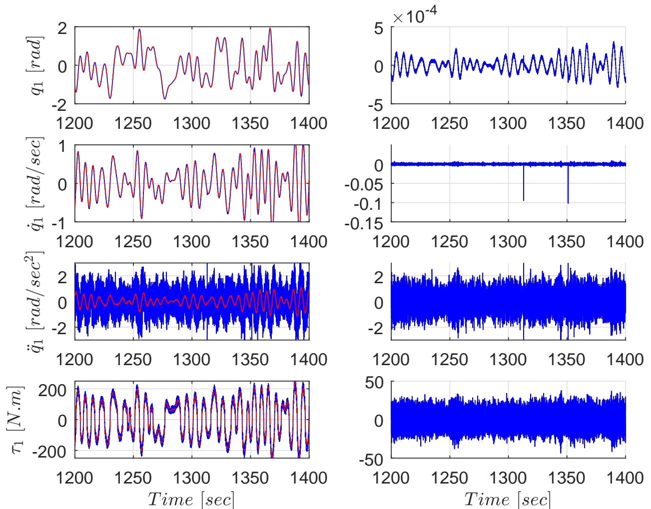
Figure 3: Data for axis 1 before (blue) and after (red) filtering (left), and the corresponding signal errors (right).
