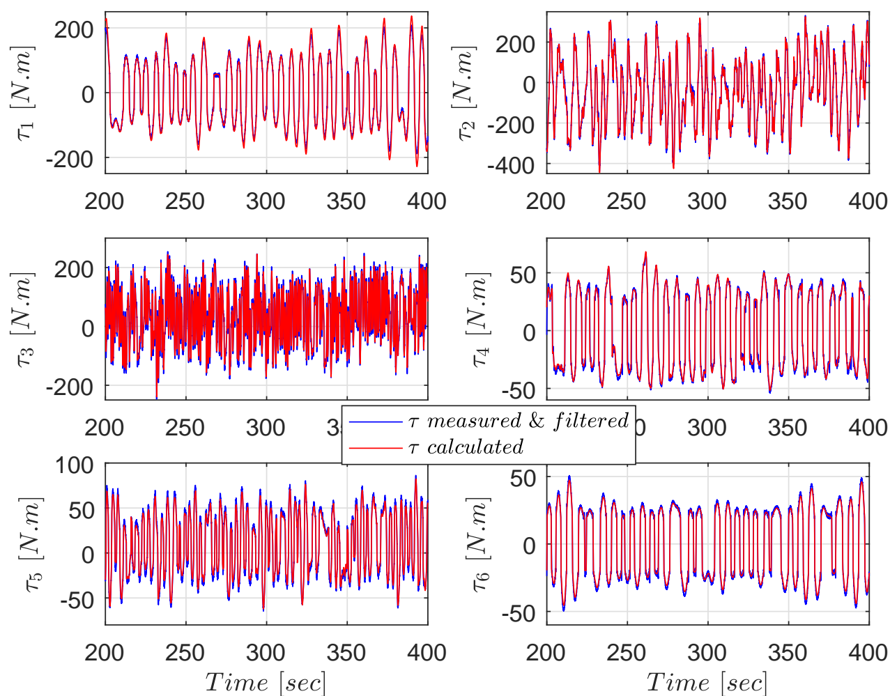
Figure 4: The filtered measured and computed torques.
