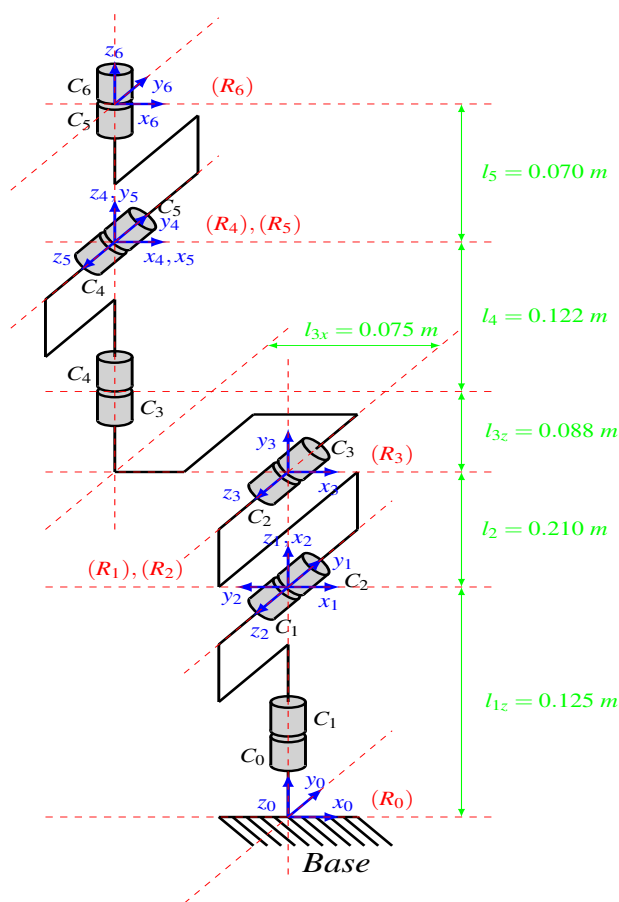
Figure 2: Robot frames for MDH convention.
