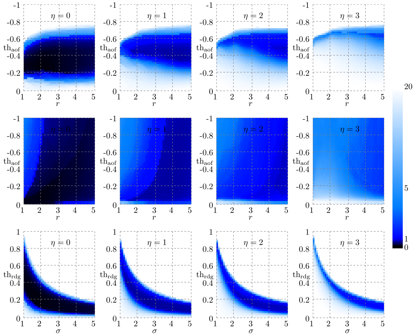
Figure 15: Modified Hausdorff distance between ground truth skeleton and computed skeleton, averaged over all shapes, versus parameter and threshold, at 4 different noise levels. Top row: AOF, middle row: CC-AOF, bottom row: ridgeness
