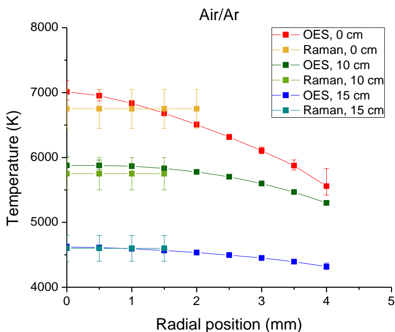
Figure 5: Temperature profiles measured with Raman scattering and OES at 0, 10 and 15 cm for the Air/Ar plasma.
